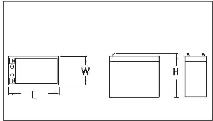
Model B-7R
