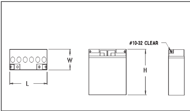
Model B-17R
